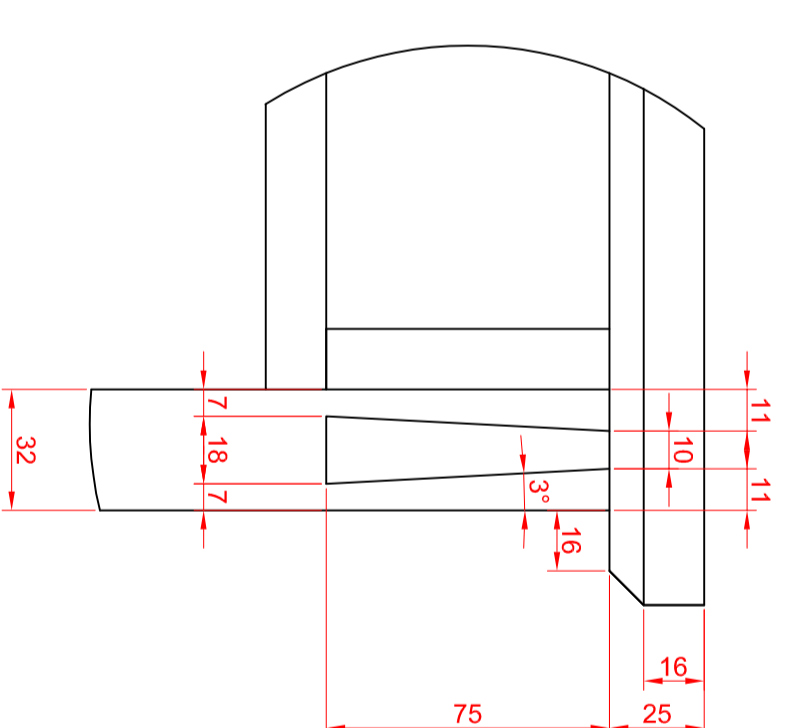
F (1:2)
